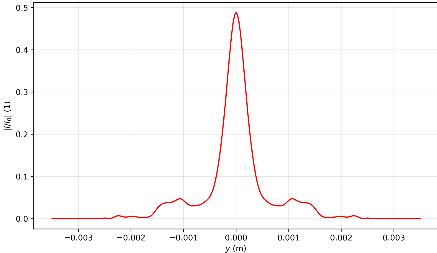
Intensity profile I(x=0, y, z=3.105)/I_0 , P_{in}=5.0P_{cr} , artificial time
